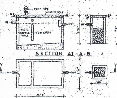
DETAILS OF SEPTIK TANK AND SOAK PIT
